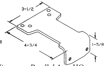
Parallel Arm Installation
