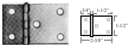
H6170 Extension Hinge Loose Pin Brass Finish Price per pair
