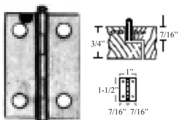
H6165 Inter-Panel Hinge, Loose Pin Brass Finish Price per pair
