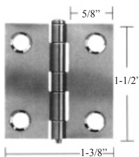
H6148 Mortise Hinge Loose Pin Brass or Nickel Price per pair
