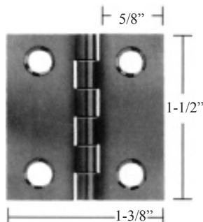
H6144 Inter-panel Hinge Tight Pin Brass Finish Price per pair
