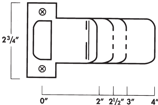
2-3/4" Extended Lip T-Strike (ETS)
