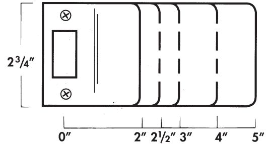
2-3/4" Extended Lip Strike (EL-2)
